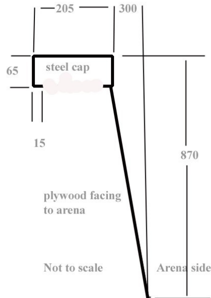
Section of arena “wall” typical
